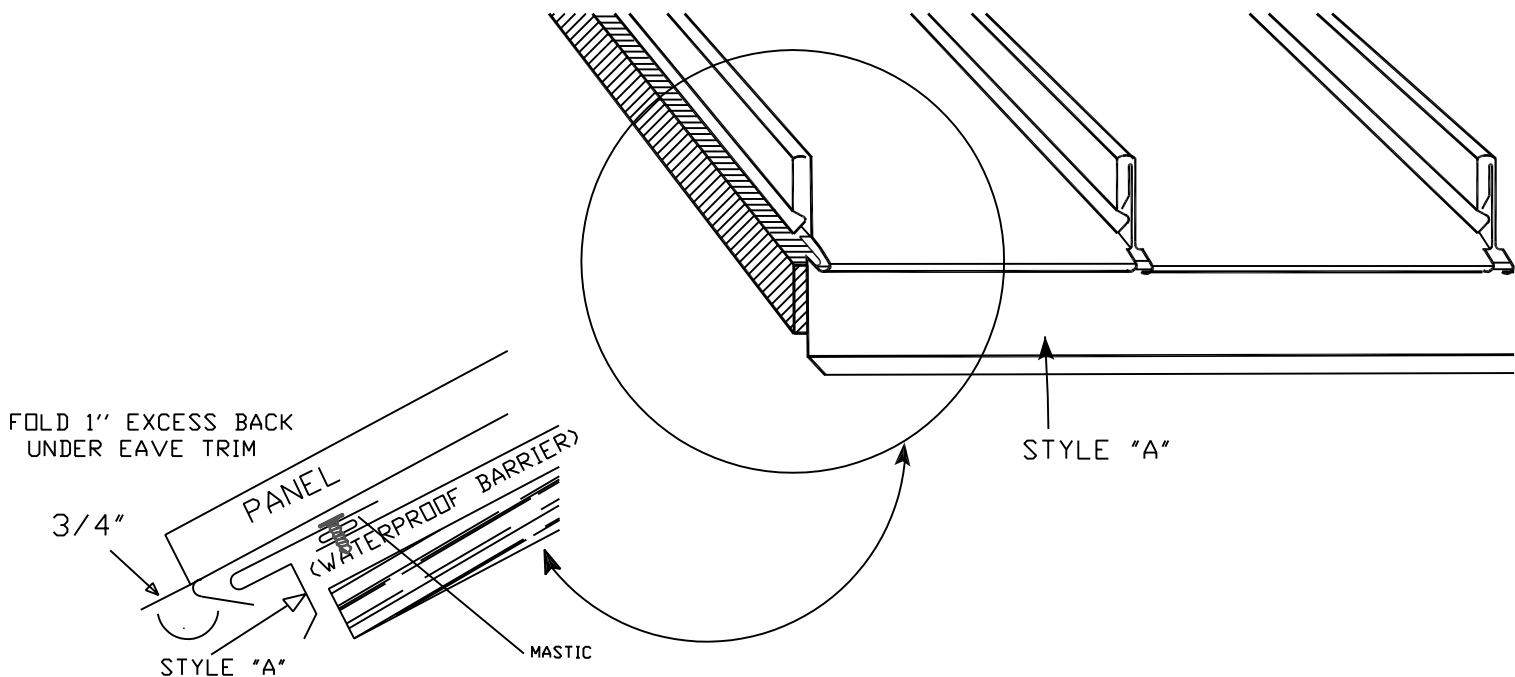
STYLE "A" EAVE TRIM CLOSED HEM
