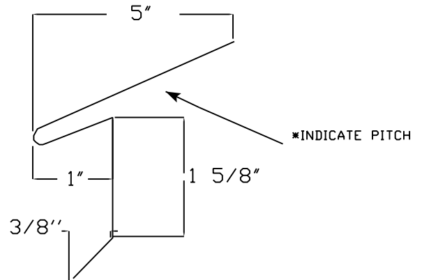
STYLE "A" EAVE TRIM CLOSED HEM
